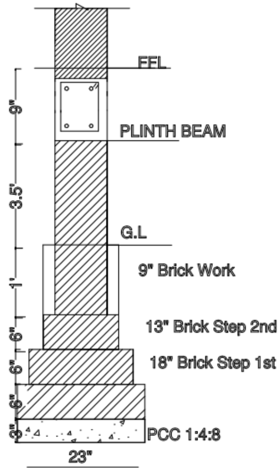
Foundation Detail
