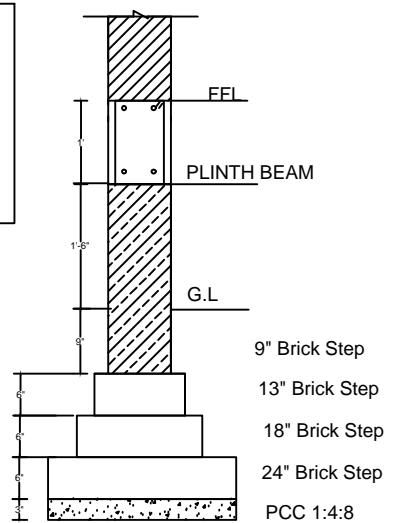
9" Wall Section
