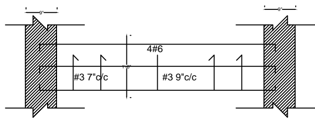
Beams Detail
